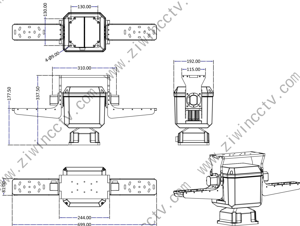
Side-Mounted Payload Dimension Drawing
