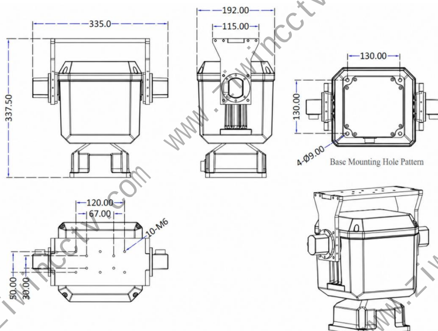
Top-Mounted Payload Dimension Drawing
